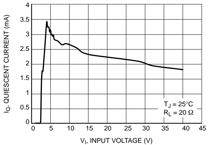
Figure 18. Quiescent Current vs. Input Voltage
