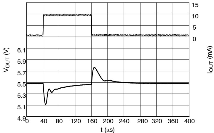
Figure 29. Load Transients, 5.5 V Version, Load Step 1 mA to 10 mA, V_{IN} = 6.5 V
