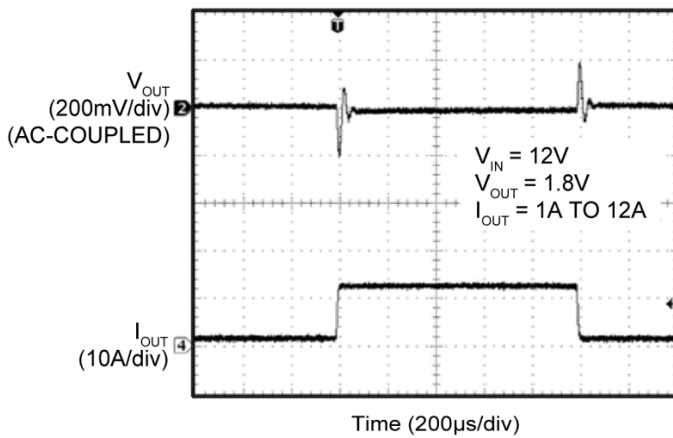
Transient Response
