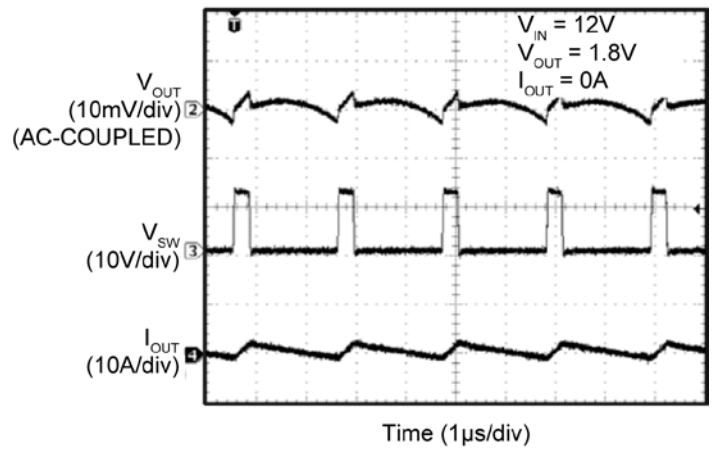
Switching Waveforms
