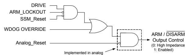
Figure 38. Arming Logic
