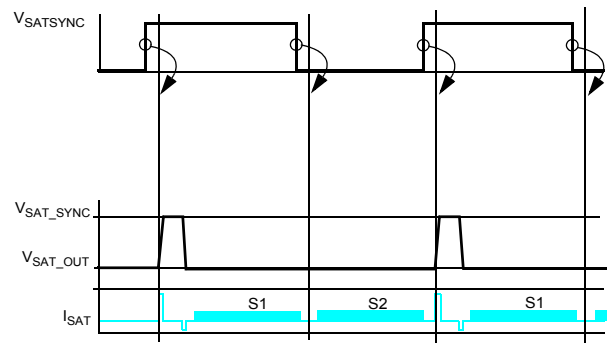
Figure 43. Satsync-steered Mode
