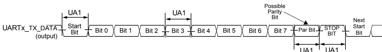
Figure 44. UART RS-232 Serial Mode Transmit Timing Diagram
