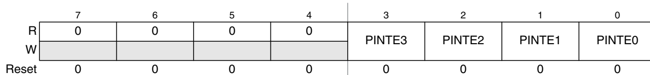
Figure 18-7. PIT Interrupt Enable Register (PITINTE)
