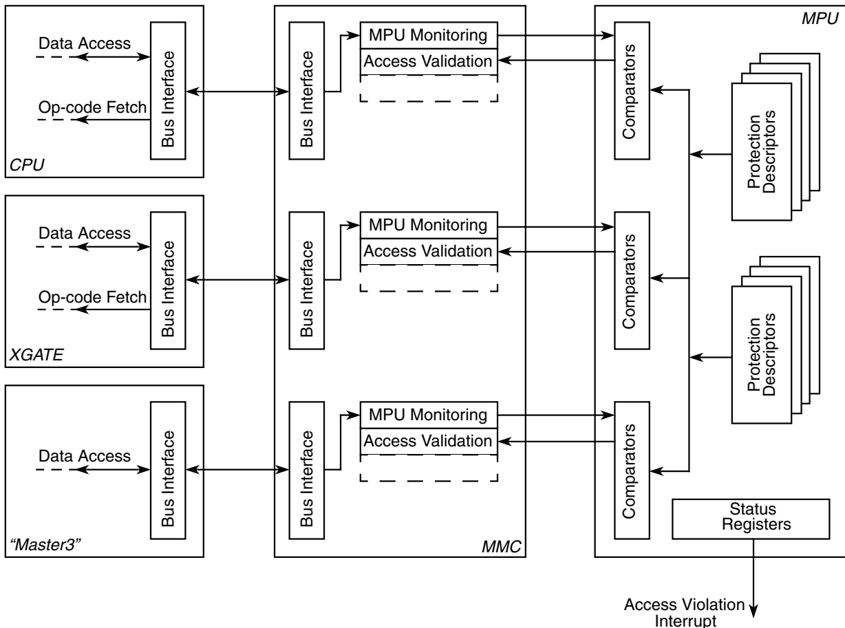
Figure 4-1. Block Diagram
