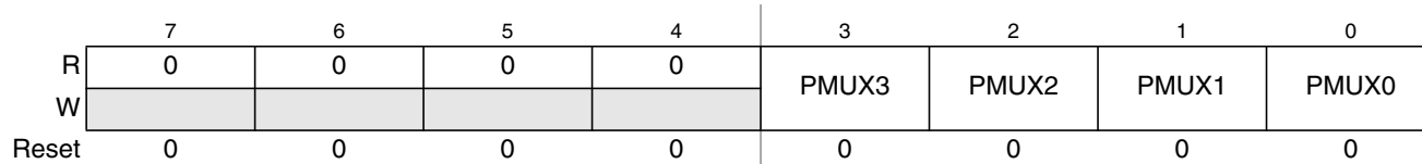
Figure 18-6. PIT Multiplex Register (PITMUX)
