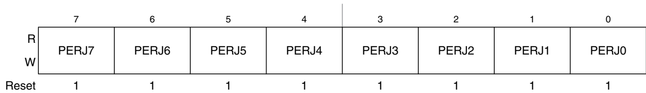
Figure 2-63. Port J Pull Device Enable Register (PERJ)
