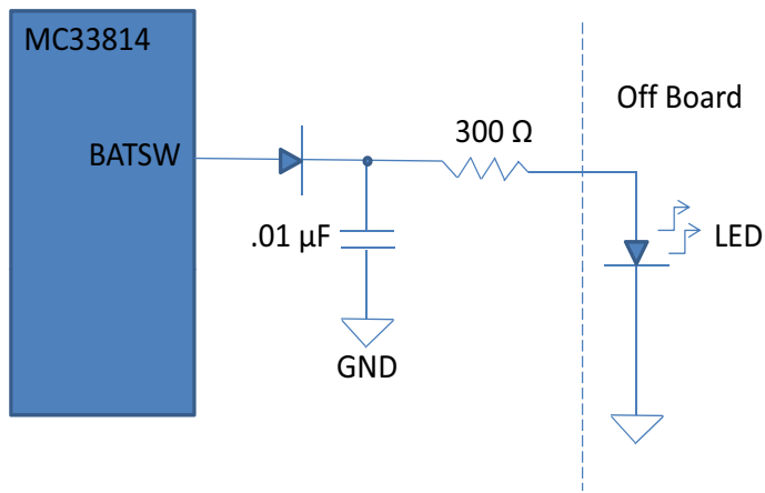
Figure 13. Recommended Circuit to Use BATSU as an LED Driver
