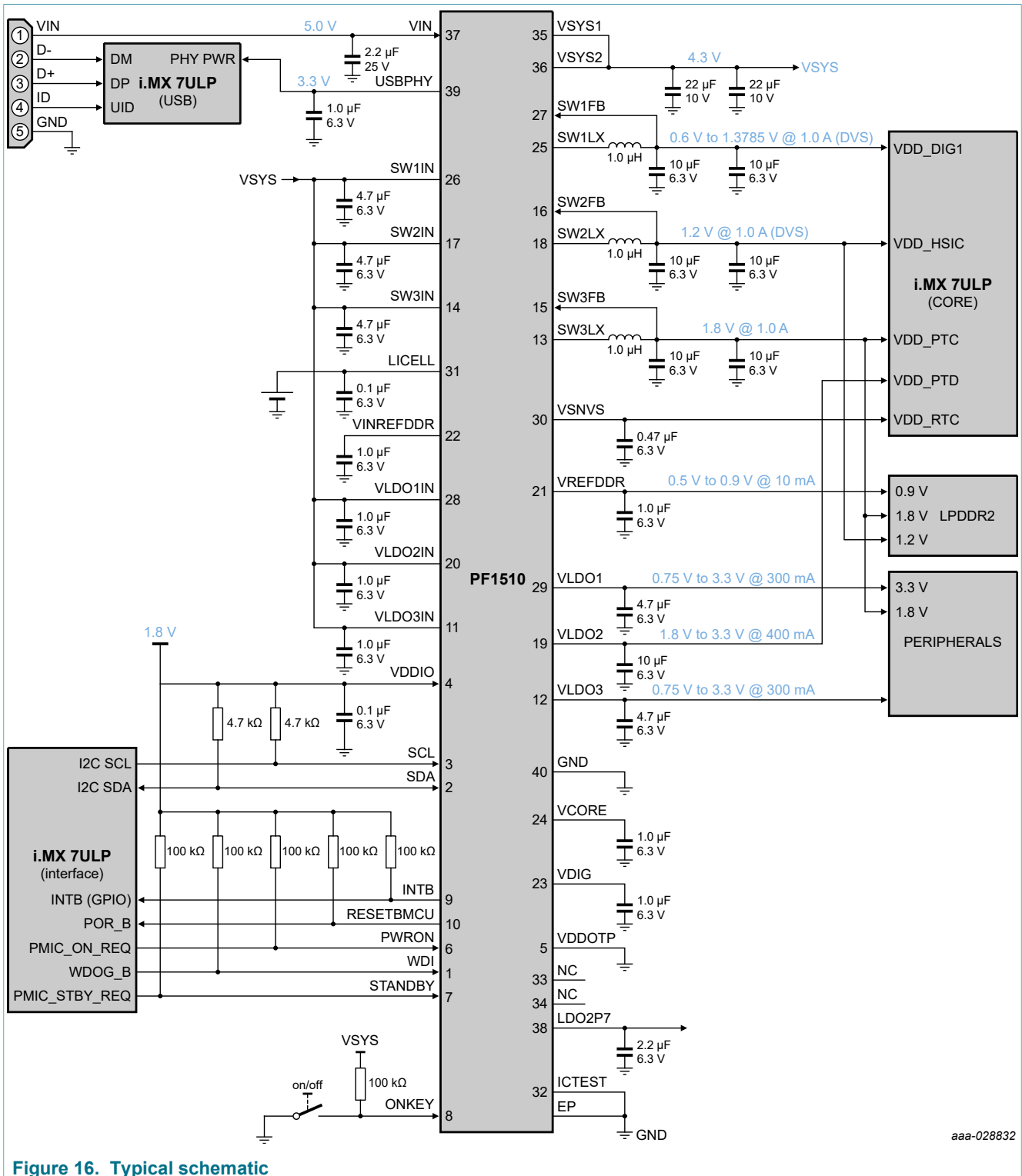
Figure 16. Typical schematic
