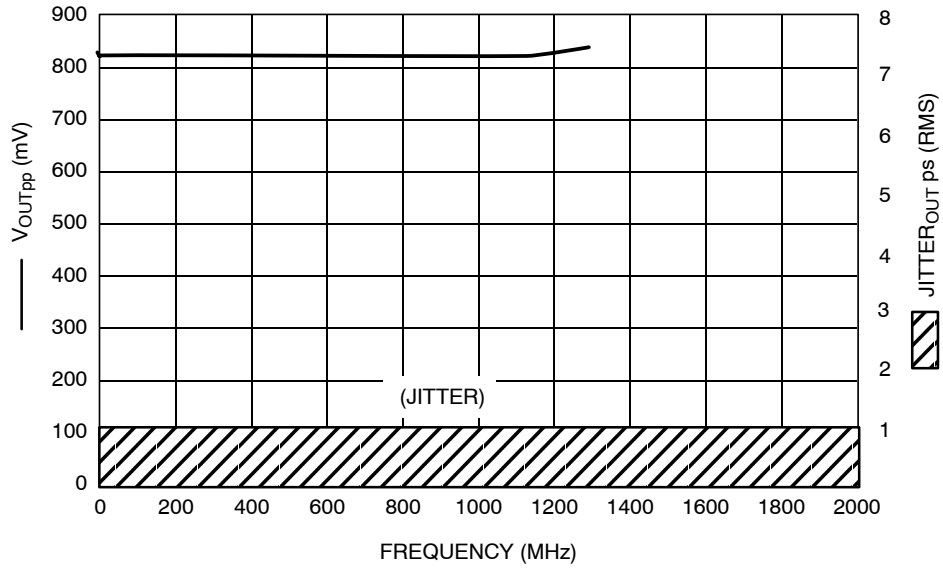
Figure 8. ÷ 4, F max /Jitter
