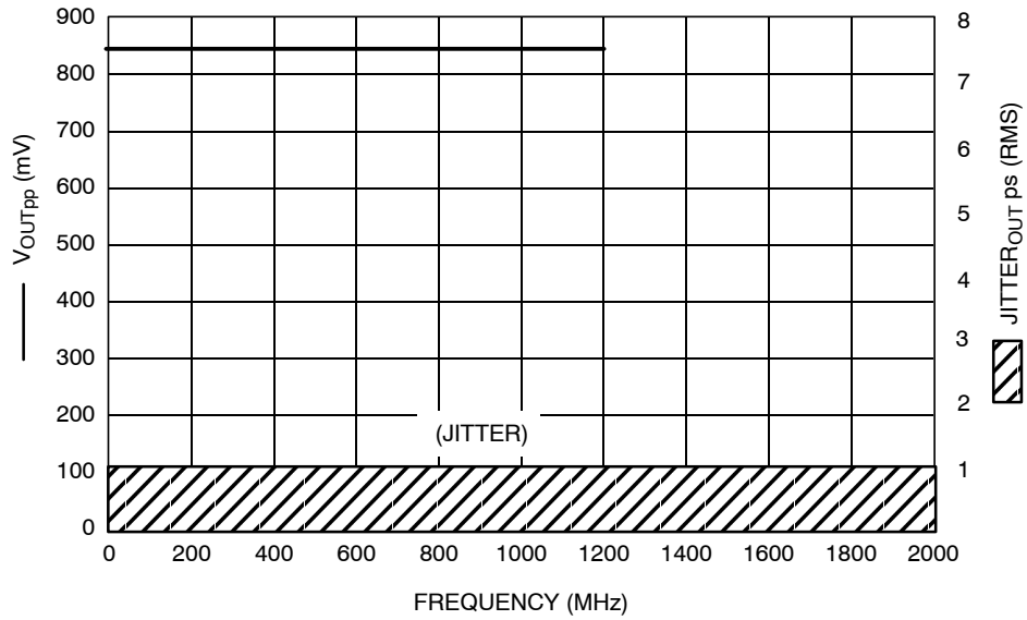
Figure 9. ÷ 6, F max /Jitter
