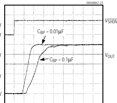
5 \mu\text{s}/\text{div} I_{LOAD} = 50\text{mA}
