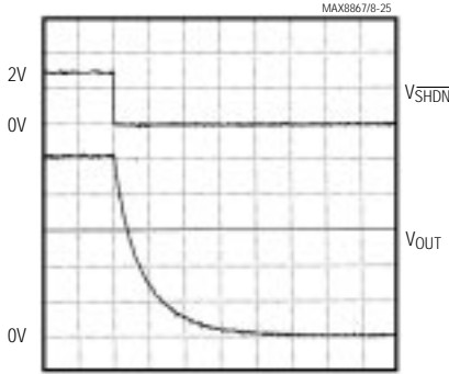
500 \mu\text{s}/\text{div} NO LOAD
