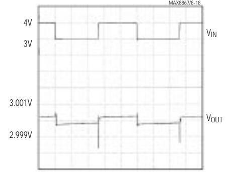
100 \mu\text{s}/\text{div} MAX886_EUK30, I_{LOAD} = 50\text{mA}
