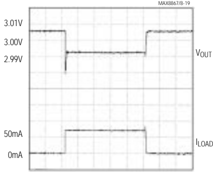
10 \mu\text{s}/\text{div} MAX886_EUK30, V_{IN} = V_{OUT} + 0.5\text{V} , C_{IN} = 10\mu\text{F} , I_{LOAD} = 0\text{mA TO } 50\text{mA}
