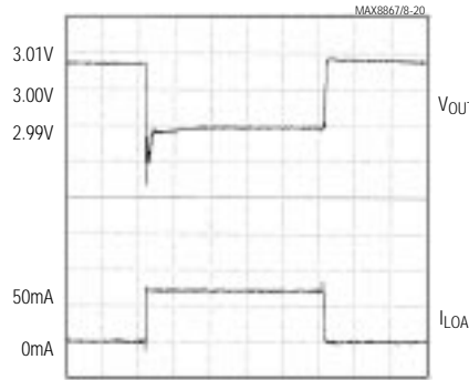
10 \mu\text{s}/\text{div} MAX886_EUK30, V_{IN} = V_{OUT} + 0.1\text{V} , C_{IN} = 10\mu\text{F} , I_{LOAD} = 0\text{mA TO } 50\text{mA}
