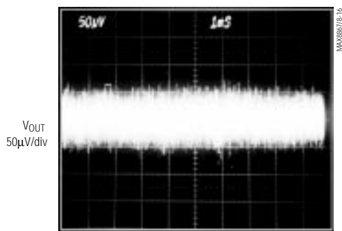
1ms/div C_{OUT} = 10\mu\text{F} , C_{BP} = 0.1\mu\text{F} , I_{LOAD} = 10\text{mA}
