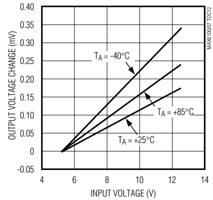
MAX6105 LINE REGULATION
