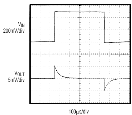
MAX6105 LINE-TRANSIENT RESPONSE
