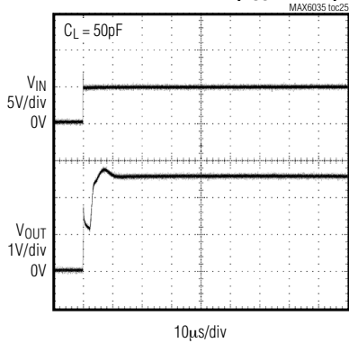
MAX6035 TURN-ON TRANSIENT ( V_{OUT} = 2.5V )
