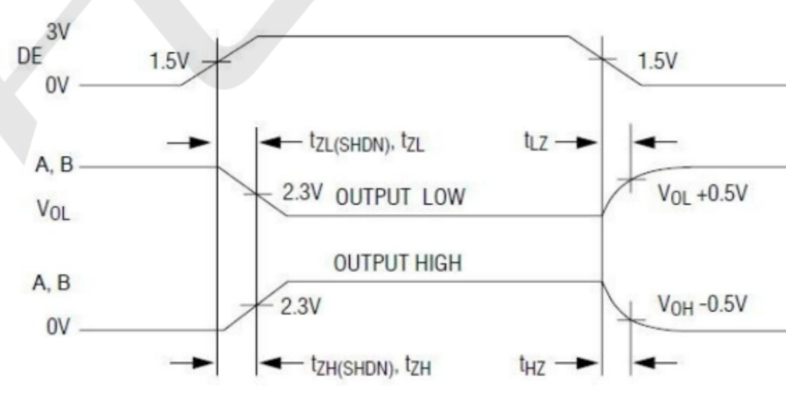
Figure 6. Driver Enable and Disable Times
