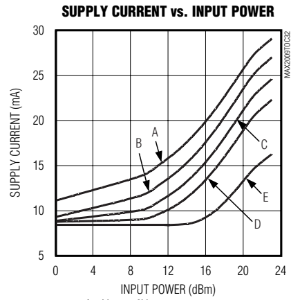
A = V_{GBP} = 0V D = V_{GBP} = 1.5V B = V_{GBP} = 0.5V E = V_{GBP} = 3.0V C = V_{GBP} = 1.0V
