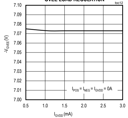
GVEE LOAD REGULATION
