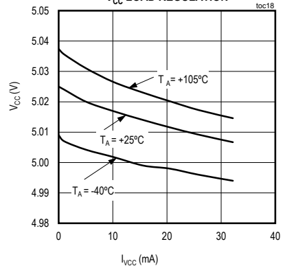
V_CC LOAD REGULATION
