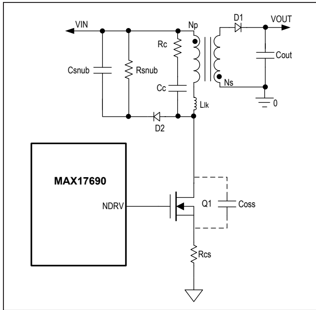
Figure 4. RC and RCD Clamp Circuitry
