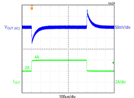
LOAD TRANSIENT BETWEEN 2A AND 4A FIGURE 3 AND FIGURE 5 CIRCUITS
