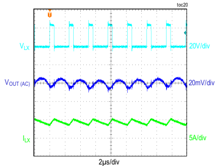
STEADY-STATE PERFORMANCE FIGURE 4 AND FIGURE 6 CIRCUITS
