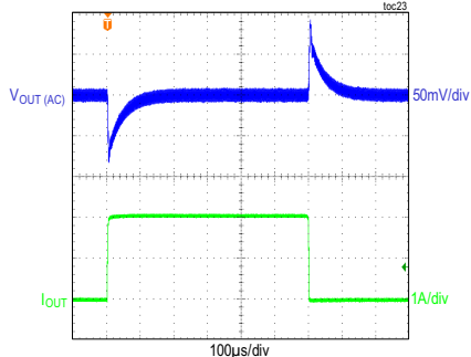
LOAD TRANSIENT BETWEEN 0A AND 2A FIGURE 3 AND FIGURE 5 CIRCUITS
