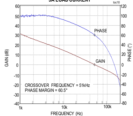
BODE PLOT, 3.3V OUTPUT 5A LOAD CURRENT
