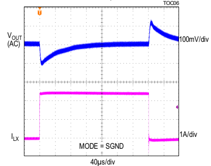
LOAD CURRENT STEPPED FROM NO LOAD TO 2.5A 3.3V OUTPUT, PWM MODE
