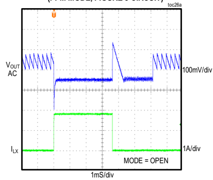
MAX17504S 5V OUTPUT LOAD CURRENT STEPPED FROM 5mA TO 1.75A (PFM MODE, FIGURE 5 CIRCUIT)
