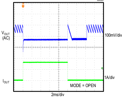
MAX17504 5V OUTPUT LOAD CURRENT STEPPED FROM 5mA TO 1.75A (PFM MODE, FIGURE 3 CIRCUIT)
