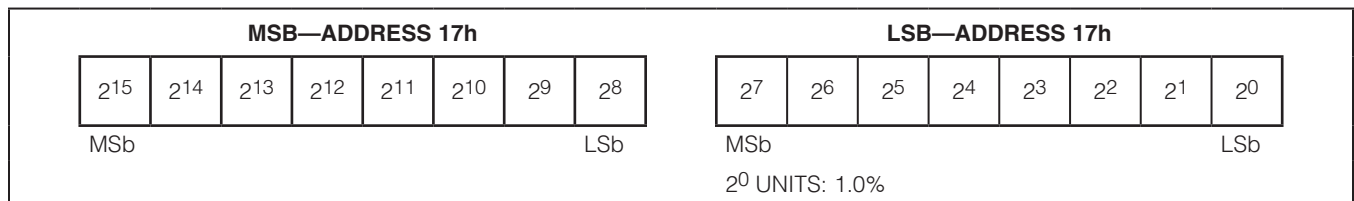
Figure 19. Cycles Register Format (Output)
