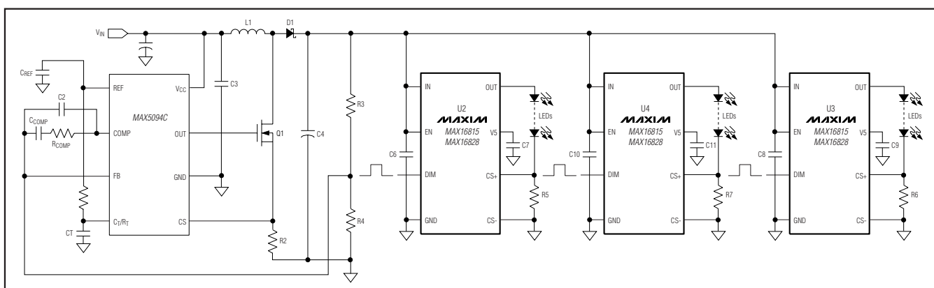
Figure 5. Multichannel HB LED Drivers for LCD Backlight
