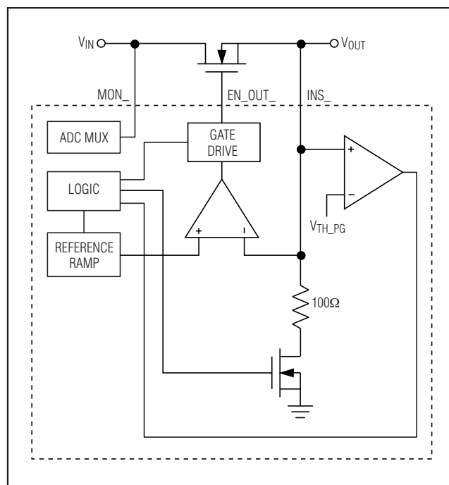
Figure 5. Closed-Loop Tracking
