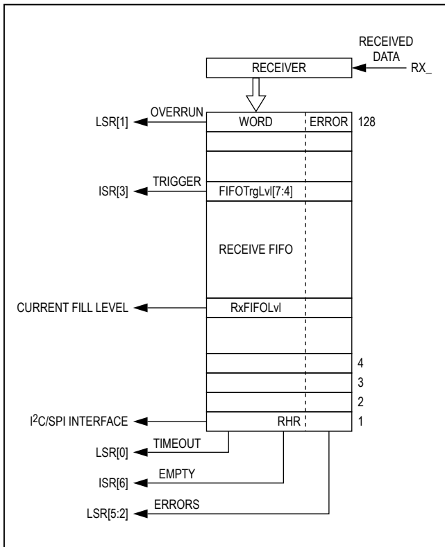
Figure 5. Receive FIFO
