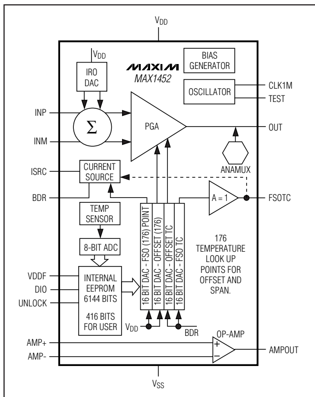
Figure 1. Functional Diagram
