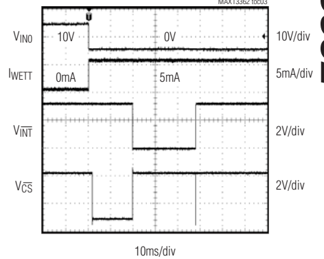
SWITCH STATUS CHANGE (CONTINUOUS MODE)
