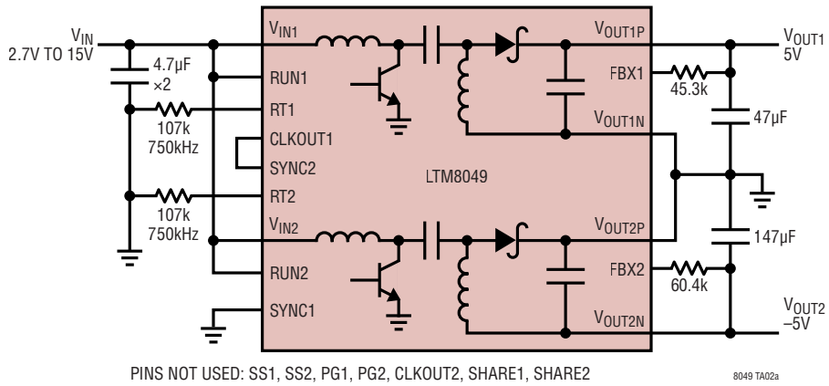
±5V Converter
