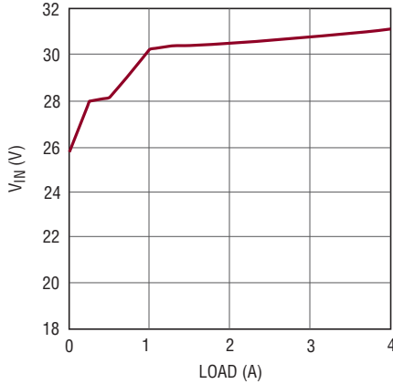
Minimum V_{IN} vs Load, V_{OUT} = 24\text{V}
