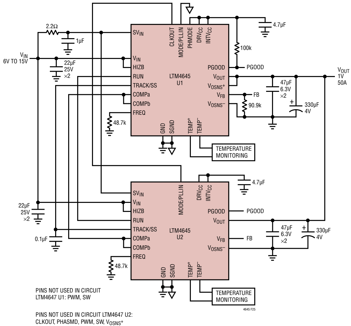
Figure 25. 6V to 15V Input, 1.0V Output at 50A
