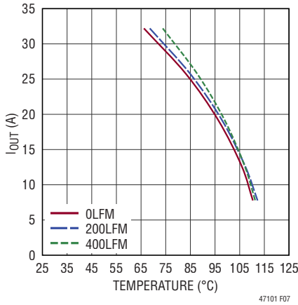
Figure 7. Derating, 4-Channel Paralleled V_{IN} = 3.3V , V_{OUT} = 0.5V DC3164A-B Demo Board
