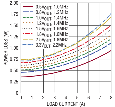
Power Loss, Single Channel V_{IN} = 5.5\text{V}
