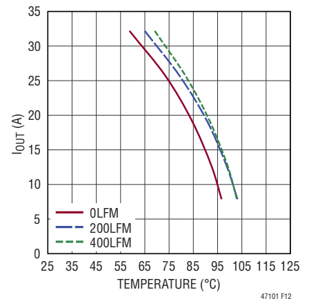
Figure 12. Derating, 4-Channel Paralleled V_{IN} = 5V , V_{OUT} = 1V DC3164A-B Demo Board
