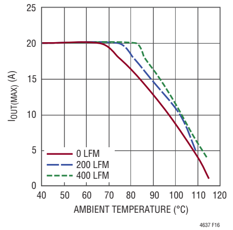
Figure 16. 5V IN to 2.5V OUT with Heat Sink
