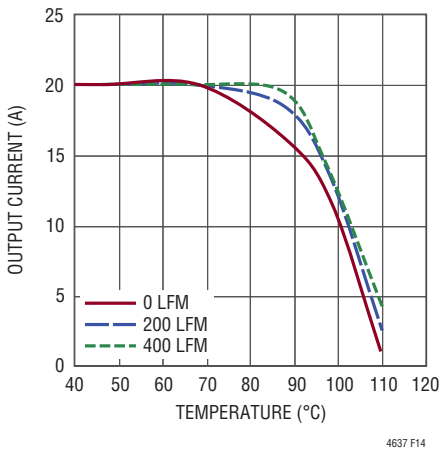
Figure 14. 12V IN to 1.0V OUT with Heat Sink
