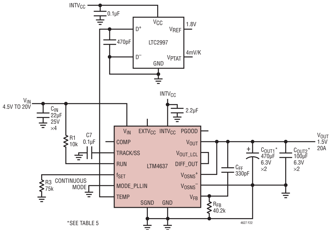
Figure 22. 4.5V to 20V IN , 1.5V at 20A Design
