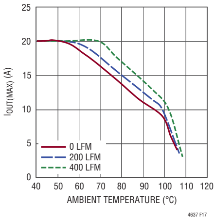
Figure 17. 12V IN to 2.5V OUT No Heat Sink
