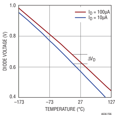
Figure 6. Diode Voltage V_D vs Temperature T(^{\circ}\text{C}) for Different Bias Currents
