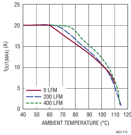
Figure 15. 5V IN to 2.5V OUT No Heat Sink
