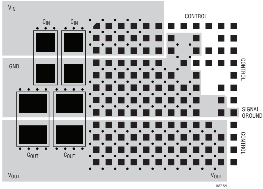
Figure 21. Recommended PCB Layout
