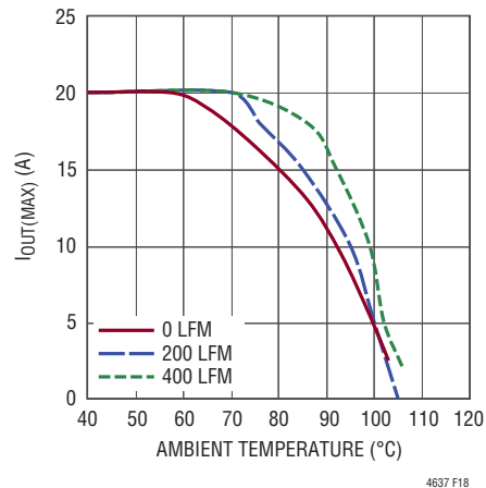
Figure 18. 12V IN to 2.5V OUT with Heat Sink
