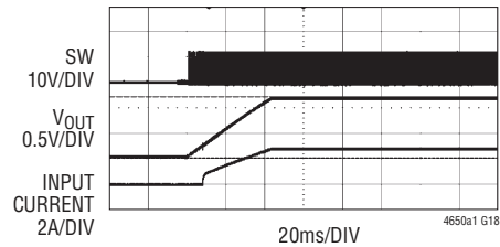
Single Phase Start-up with 25A Load
