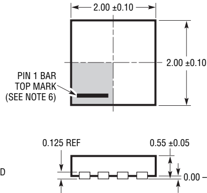
KC Package 8-Lead Plastic UTDFN (2mm × 2mm) (Reference LTC DWG # 05-08-1749 Rev 0)
