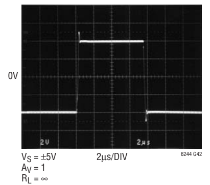
Large-Signal Response
