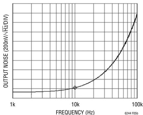
Figure 5b: Output Noise Spectral Density of Figure 5a. The Simple JFET Bootstrap Improves Noise (and Bandwidth) Drastically. Noise Density at 10kHz is Now 220\text{nV}/\sqrt{\text{Hz}} , About a 8.2x Reduction. This is Mostly Due to the Bootstrap Effect of Swapping the 1\text{nV}/\sqrt{\text{Hz}} of the JFET for the 7.8\text{nV}/\sqrt{\text{Hz}} of the Op Amp
