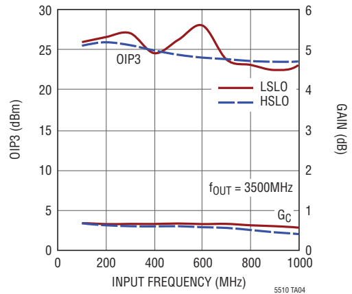
Conversion Gain and OIP3 vs Input Frequency
