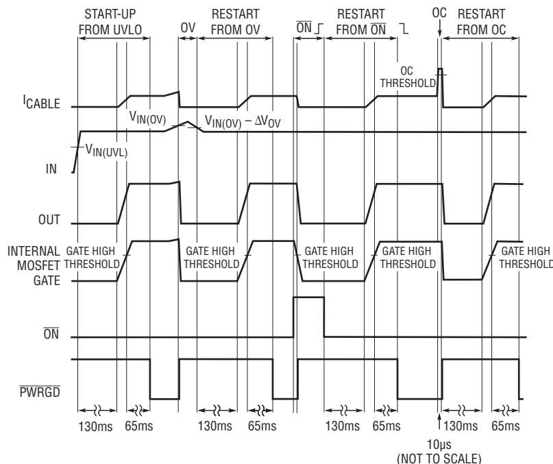
Figure 2. \overline{PWRGD} Behavior
