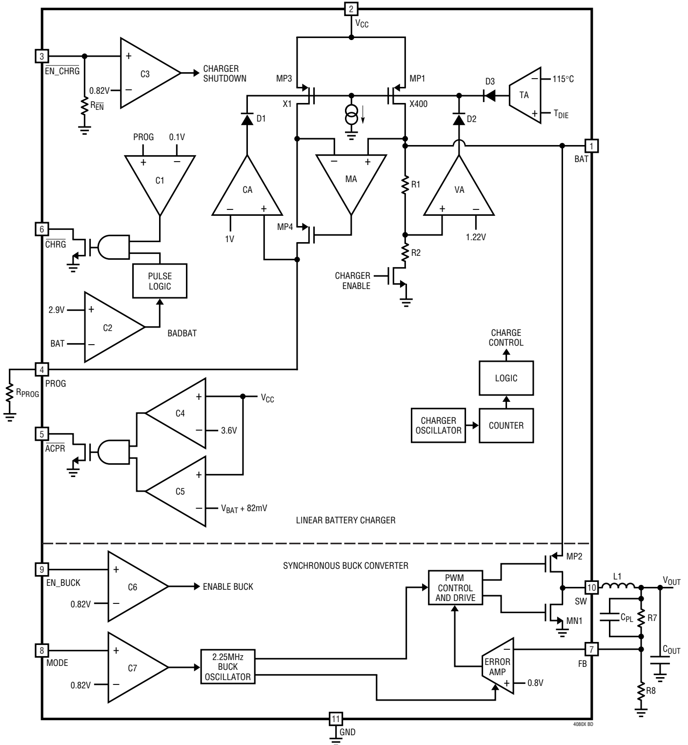
Figure 1. LTC4080X Block Diagram
