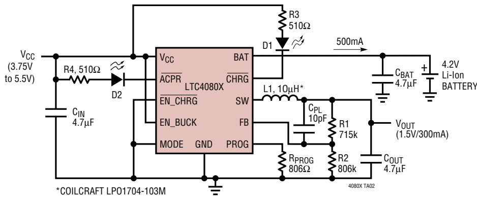
Li-Ion Battery Charger with 1.5V Buck Regulator
