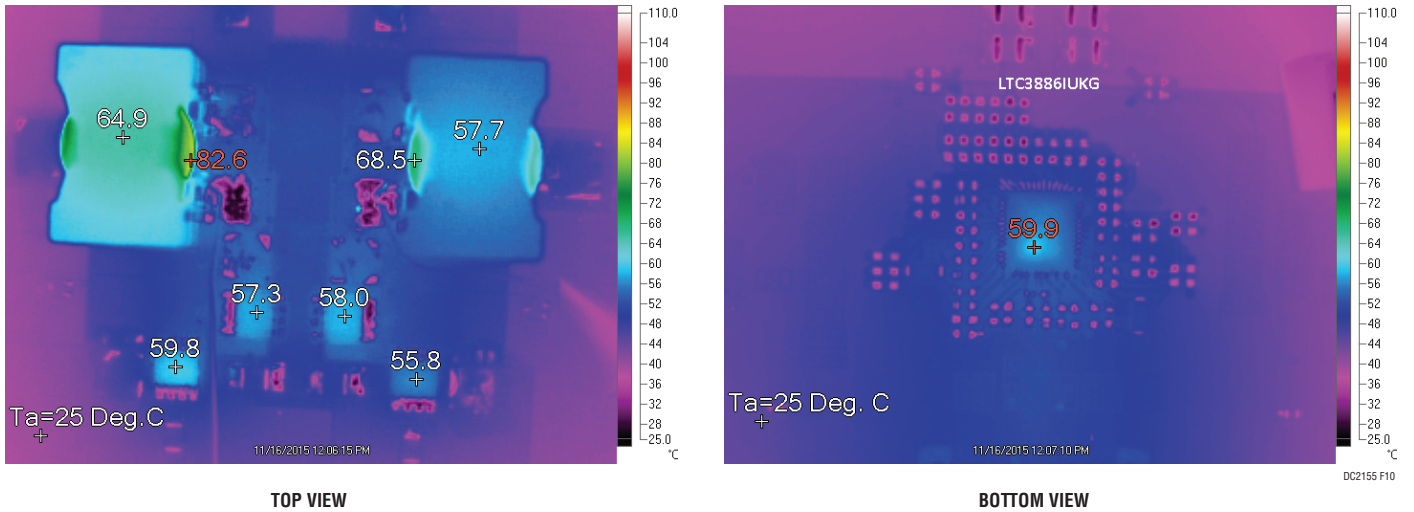
V_{IN} = 32V V_{OUT0} = 12V \text{ AT } 12A V_{OUT1} = 5V \text{ AT } 12A f_{SW} = 150kHz EXTV_{CC} = 12V \text{ (TIED TO } V_{OUT}) T_A = 25^\circ C NO FORCED AIRFLOW (DEFAULT SET-UP)
