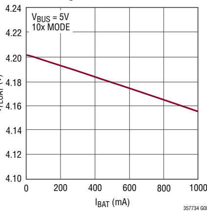
Battery Float Voltage Load Regulation
