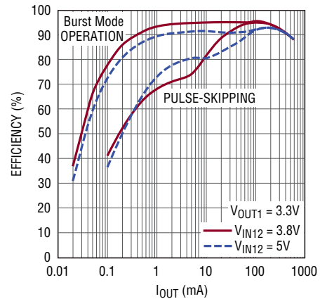
Step-Down Switching Regulator 1 3.3V Output Efficiency vs I_{\text{OUT}1}
