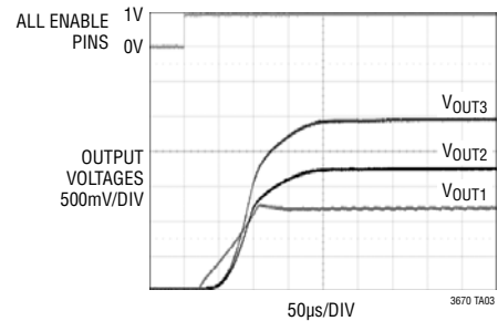
Start-Up Transient
