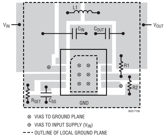
Figure 10. Layout Example
