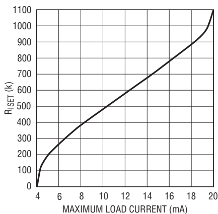
Figure 1. R_{ISET} Selection
