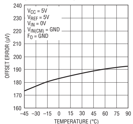
Offset Error vs Temperature (2x Speed Mode)
