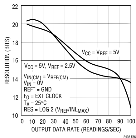
Figure 36. Resolution ( INL_{MAX} \leq 1LSB ) vs Output Data Rate and Temperature
