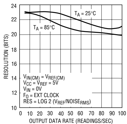
Figure 32. Resolution ( Noise_{RMS} \leq 1LSB ) vs Output Data Rate and Temperature
