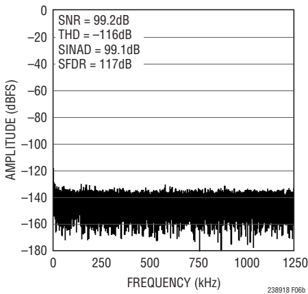
Figure 6b. 32k Point FFT f_{\text{SAMPL}} = 2.5\text{Mpsps} , f_{\text{IN}} = 2\text{kHz} , for Circuit Shown in Figure 6a; Driven with Fully Differential Inputs
