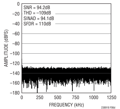
Figure 6d. 32k Point FFT f_{\text{SAMPL}} = 2.5\text{Mpsps} , f_{\text{IN}} = 2\text{kHz} , for Circuit Shown in Figure 6a; Driven with Bipolar Inputs
