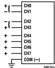
Figure 1a. Example MUX Configurations
