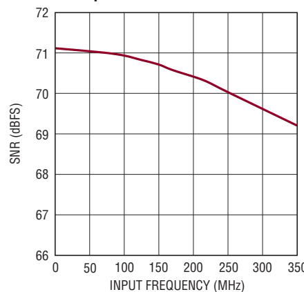
LTC2265-12: SNR vs Input Frequency, -1dBFS, 2V Range, 65Mps
