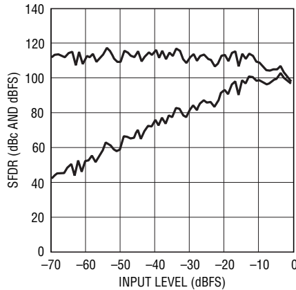
LTC2202: SFDR vs Input Level, f IN = 30.1MHz, PGA = 0, Dither "On"
