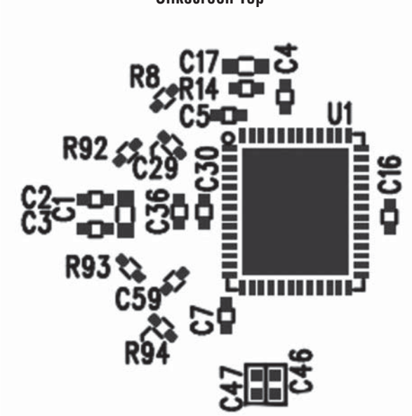
Silkscreen Top
