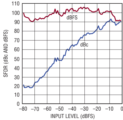
LTC2172-12: SFDR vs Input Level, f_{IN} = 70\text{MHz} , 2V Range, 65Msps
