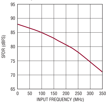
LTC2171-12: SFDR vs Input Frequency, -1dBFS, 2V Range, 40Mps
