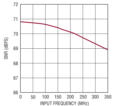
LTC2171-12: SNR vs Input Frequency, -1dBFS, 2V Range, 40Mps
