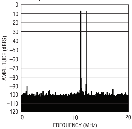
LTC2171-12: 8k Point 2-Tone FFT, f_{IN} = 68\text{MHz}, 69\text{MHz} , -1dBFS, 40Mps
