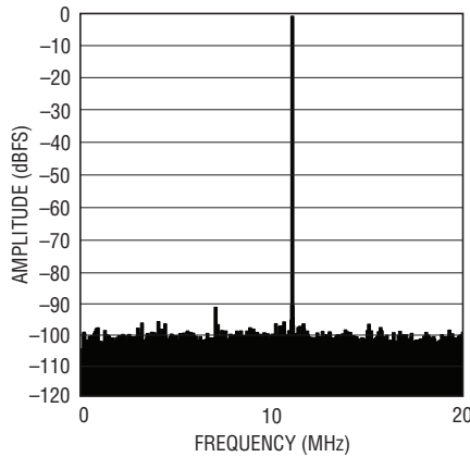
LTC2171-12: 8k Point FFT, f_{IN} = 69\text{MHz} -1dBFS, 40Mps
