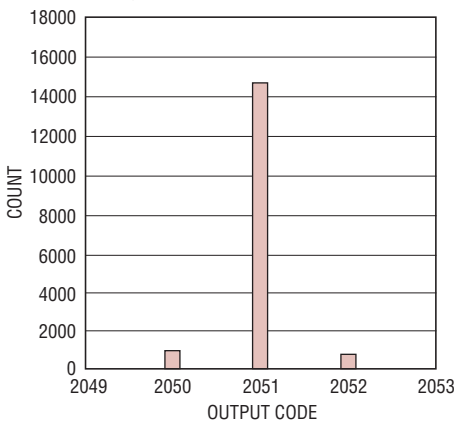
LTC2172-12: Shorted Input Histogram
