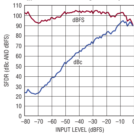
LTC2171-12: SFDR vs Input Level, f_{IN} = 70\text{MHz} , 2V Range, 40Mps
