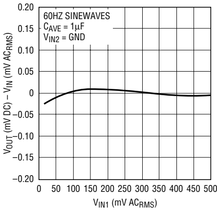
AC Linearity
