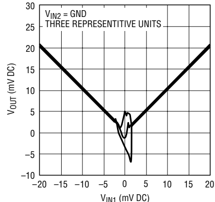
DC Transfer Function Near Zero
