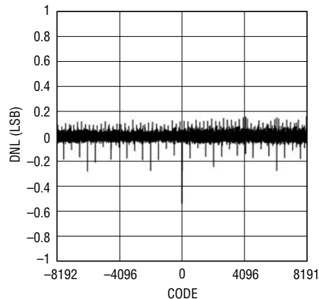
LTC1855 Typical DNL Curve
